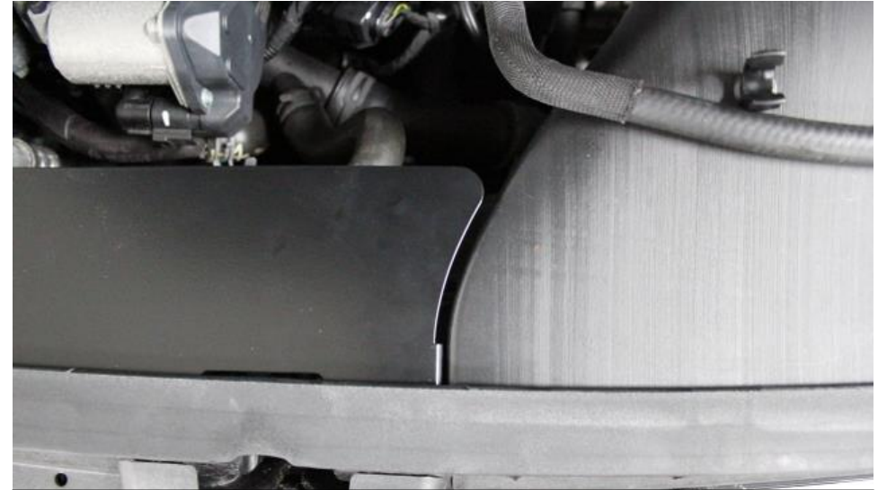
14. Adjust the height of the top panel so it sits level with the duct and then tighten the screw you used to put them together in step 9.
